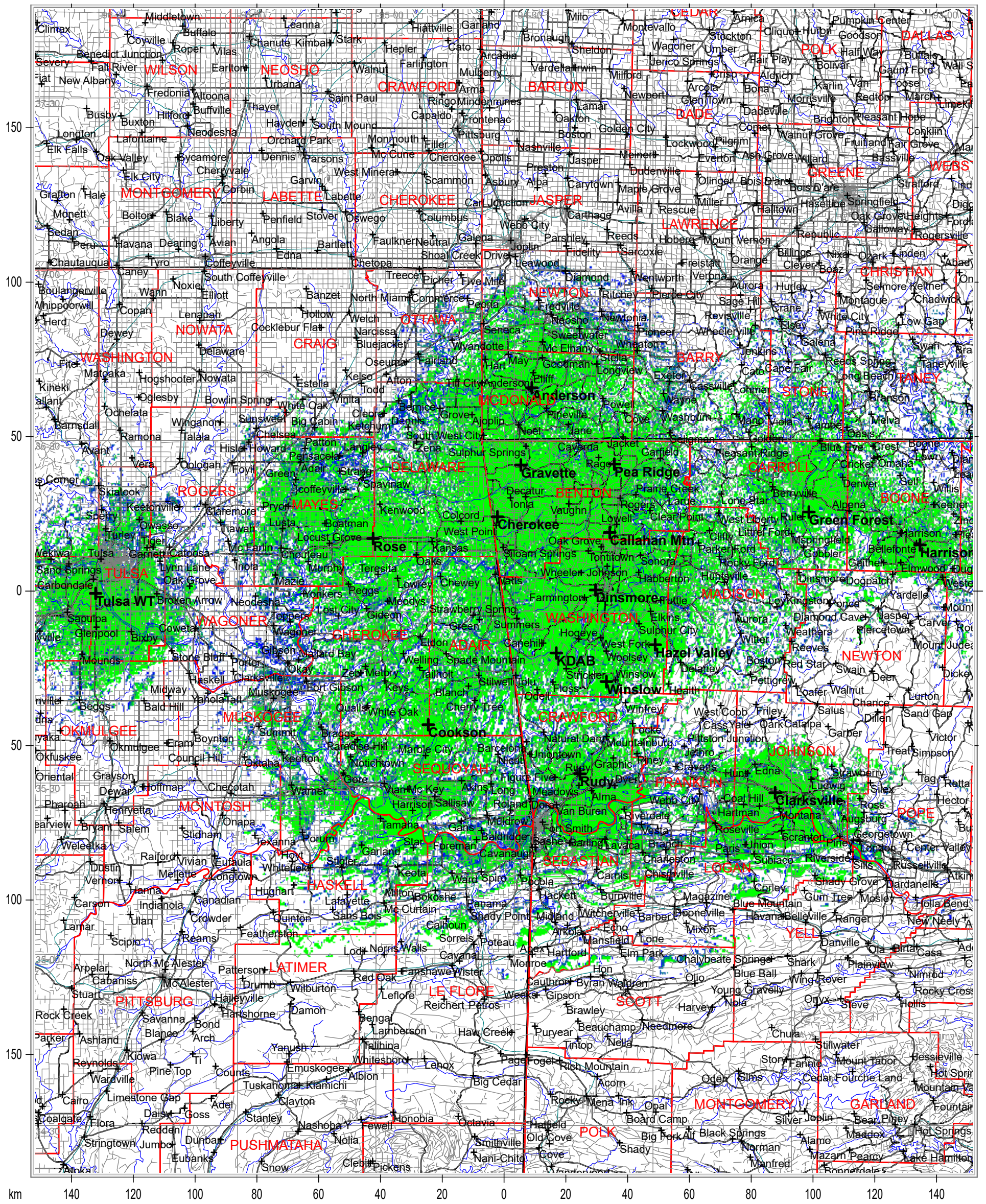
SMITH 2-WAY -- SMR UHF MOBILE TALKBACK -- 16-SITE COMPOSITE (NEXEDGE)
